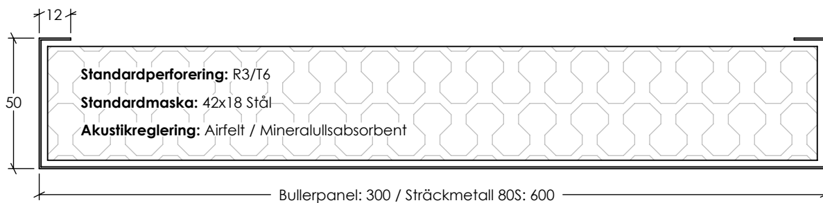
Bullerpanel / Sträckmetall 80S, L: Max 2500
